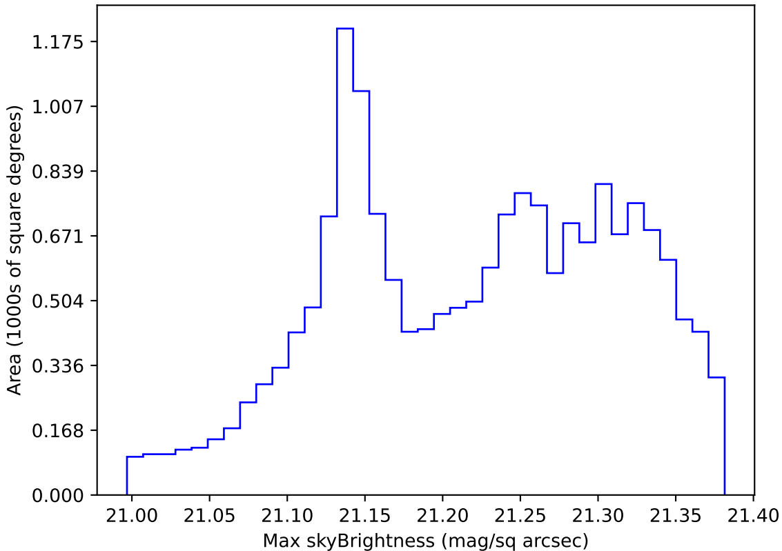
ddf_loaded_half_fl2_v3.4_10yrs WFD r band: Max skyBrightness
