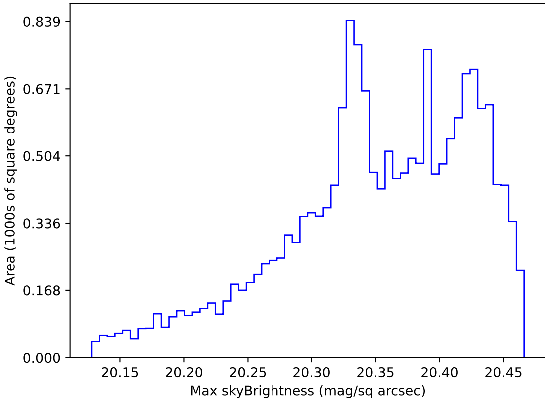
ddf_loaded_half_fl2_v3.4_10yrs WFD i band: Max skyBrightness
