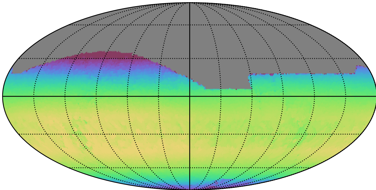
ddf_loaded_half_fl2_v3.4_10yrs All sky z band: Max skyBrightness
