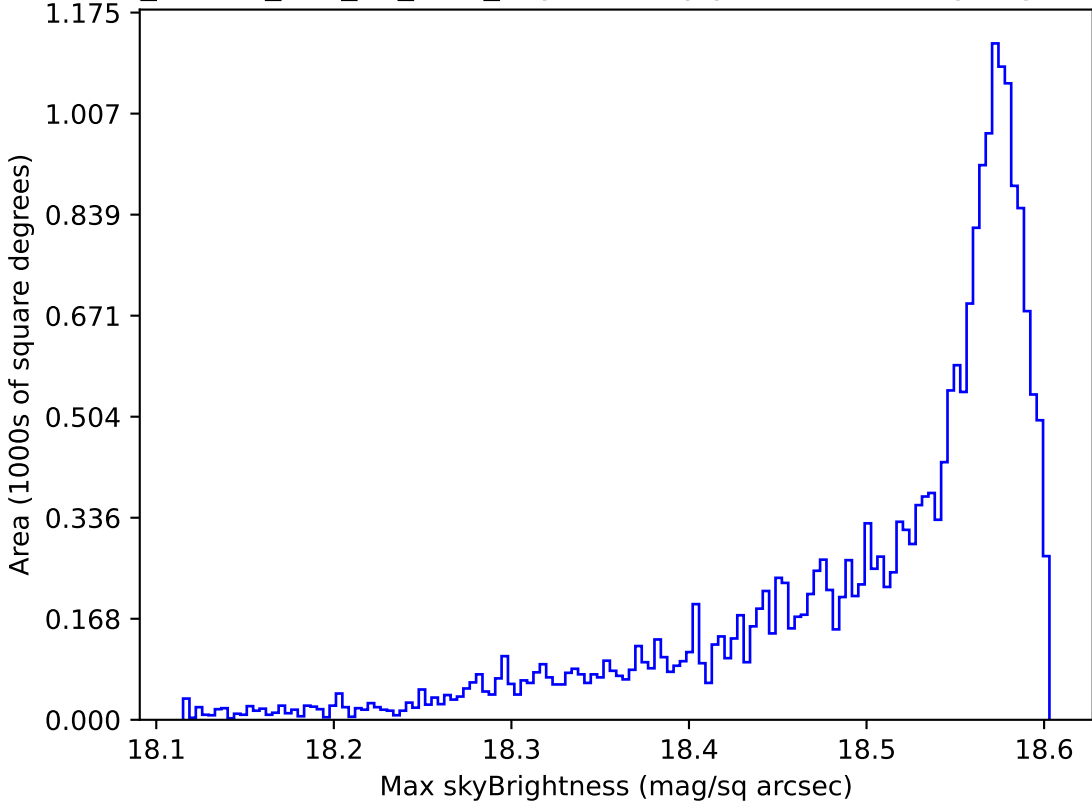
ddf_loaded_half_fl2_v3.4_10yrs All sky y band: Max skyBrightness
