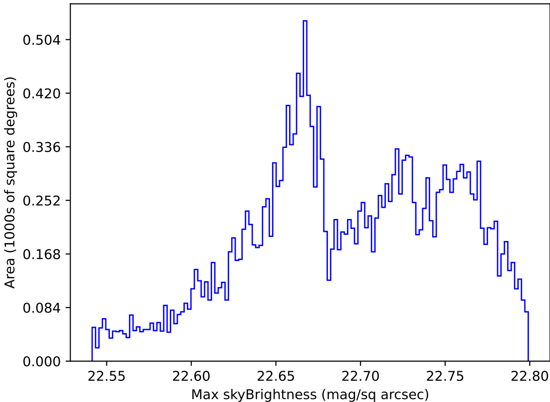
ddf_loaded_half_fl2_v3.4_10yrs All sky u band: Max skyBrightness
