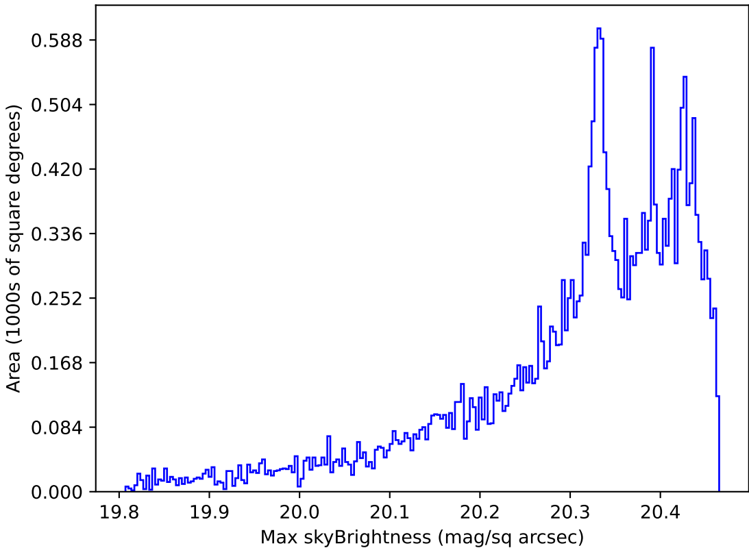
ddf_loaded_half_fl2_v3.4_10yrs All sky i band: Max skyBrightness
