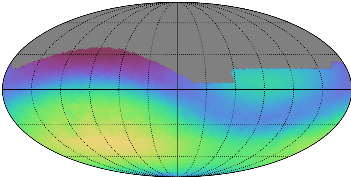
ddf_loaded_half_fl2_v3.4_10yrs All sky g band: Max skyBrightness
