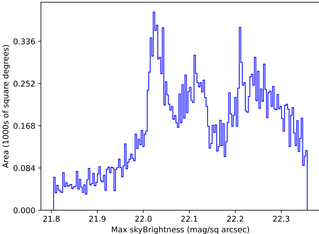
ddf_loaded_half_fl2_v3.4_10yrs All sky g band: Max skyBrightness
