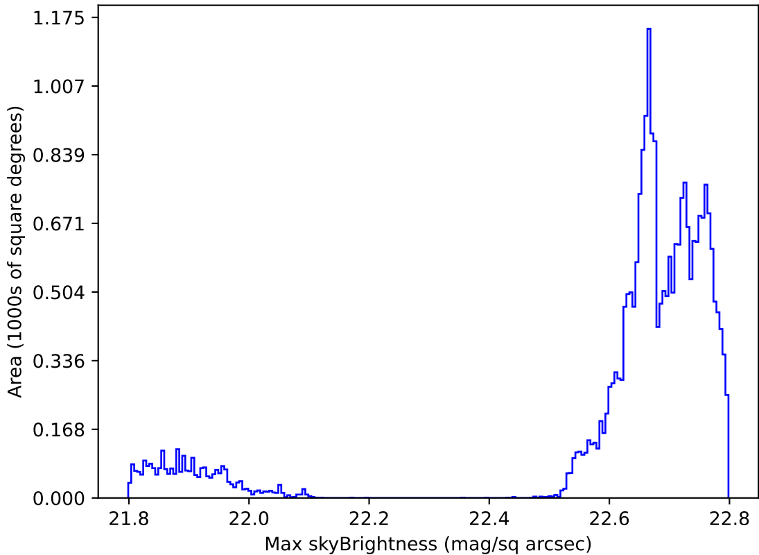
ddf_loaded_half_fl2_v3.4_10yrs All sky all bands: Max skyBrightness
