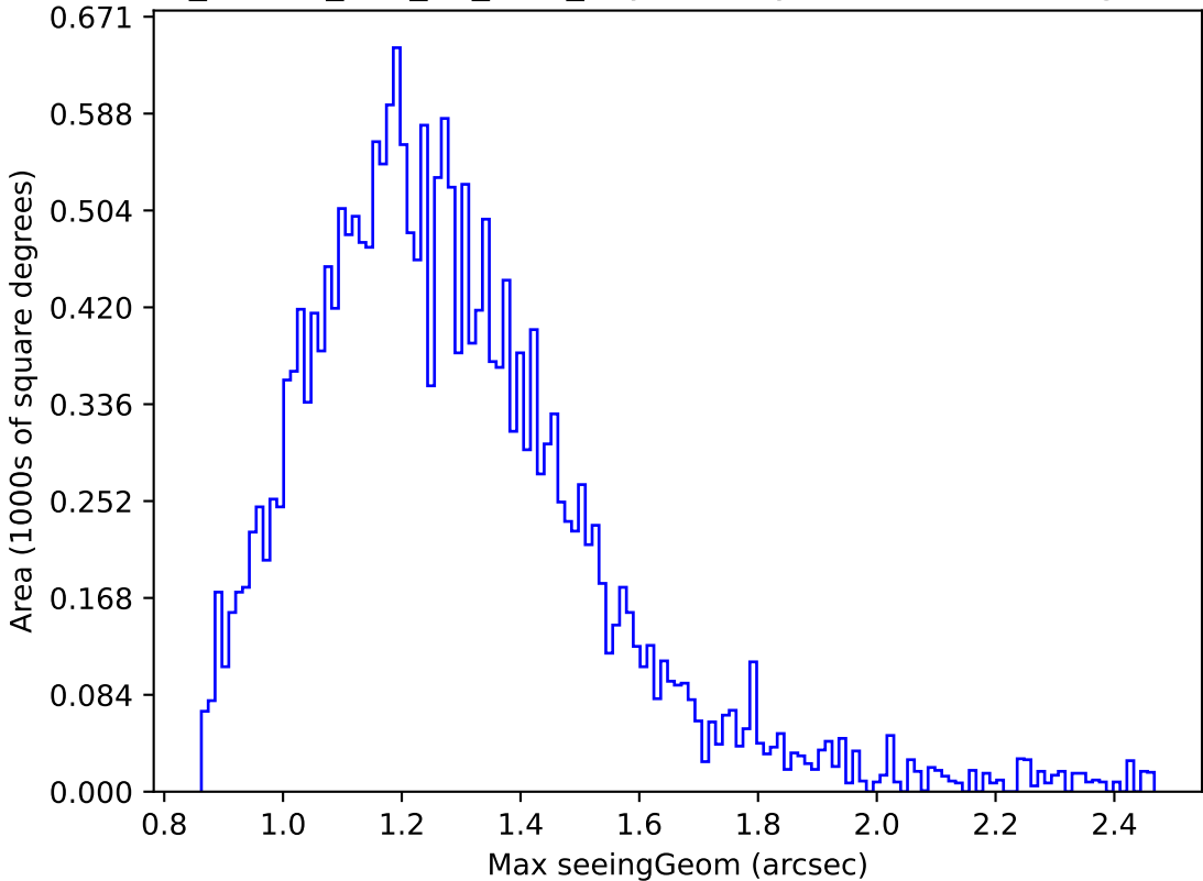
ddf_loaded_half_fl2_v3.4_10yrs Yr 1 y band: Max seeingGeom
