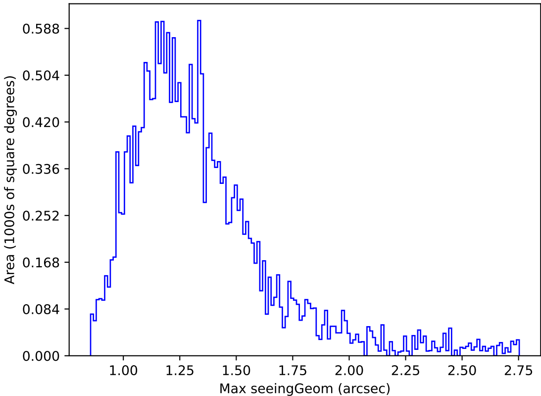
ddf_loaded_half_fl2_v3.4_10yrs Yr 1 u band: Max seeingGeom
