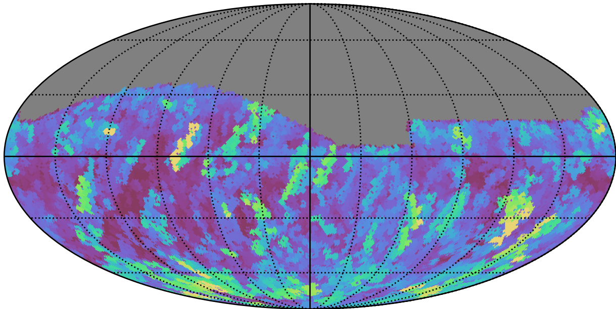
ddf_loaded_half_fl2_v3.4_10yrs Yr 1 r band: Max seeingGeom
