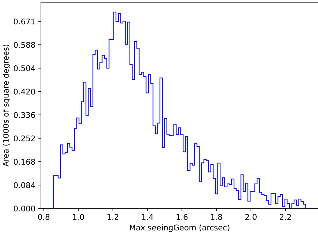
ddf_loaded_half_fl2_v3.4_10yrs Yr 1 r band: Max seeingGeom
