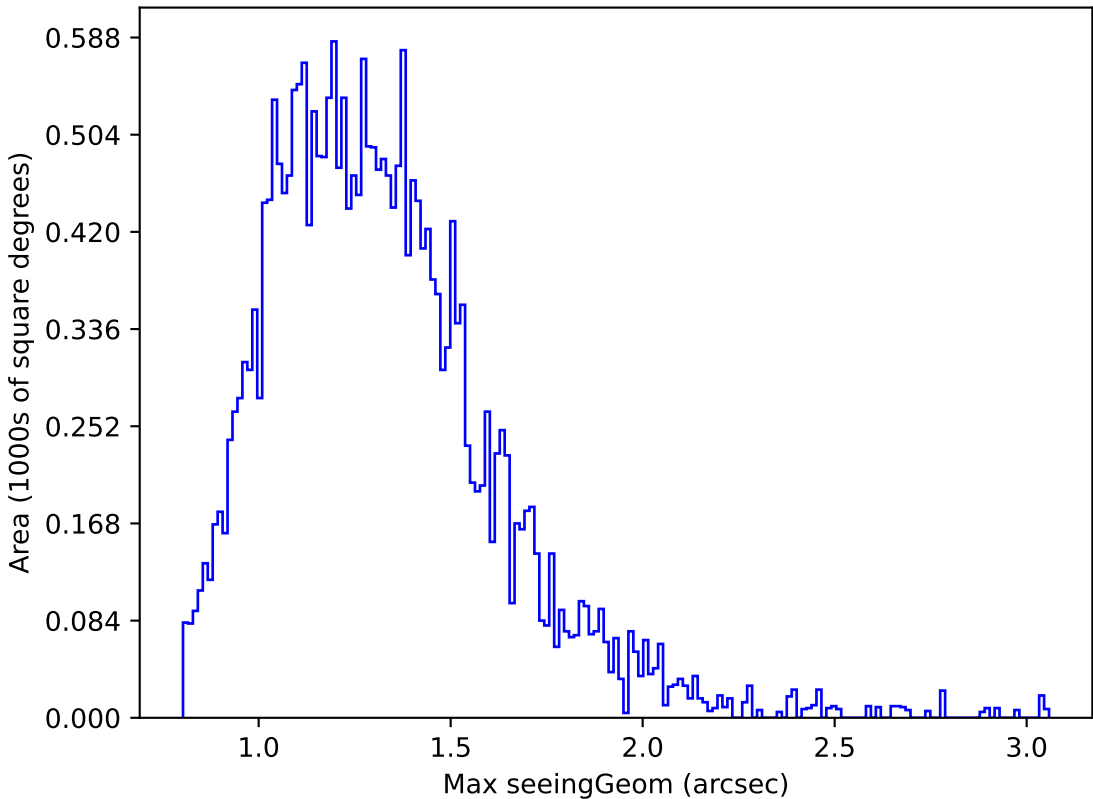
ddf_loaded_half_fl2_v3.4_10yrs Yr 1 g band: Max seeingGeom
