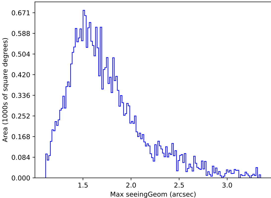
ddf_loaded_half_fl2_v3.4_10yrs Yr 1 all bands: Max seeingGeom
