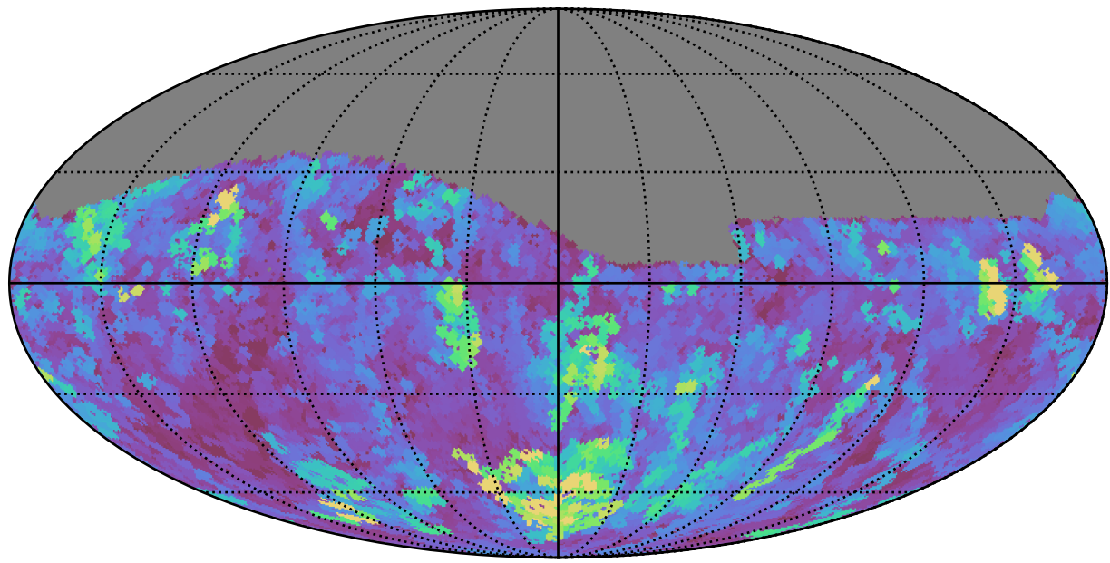
ddf_loaded_half_fl2_v3.4_10yrs Yr 1 z band: Max seeingEff
