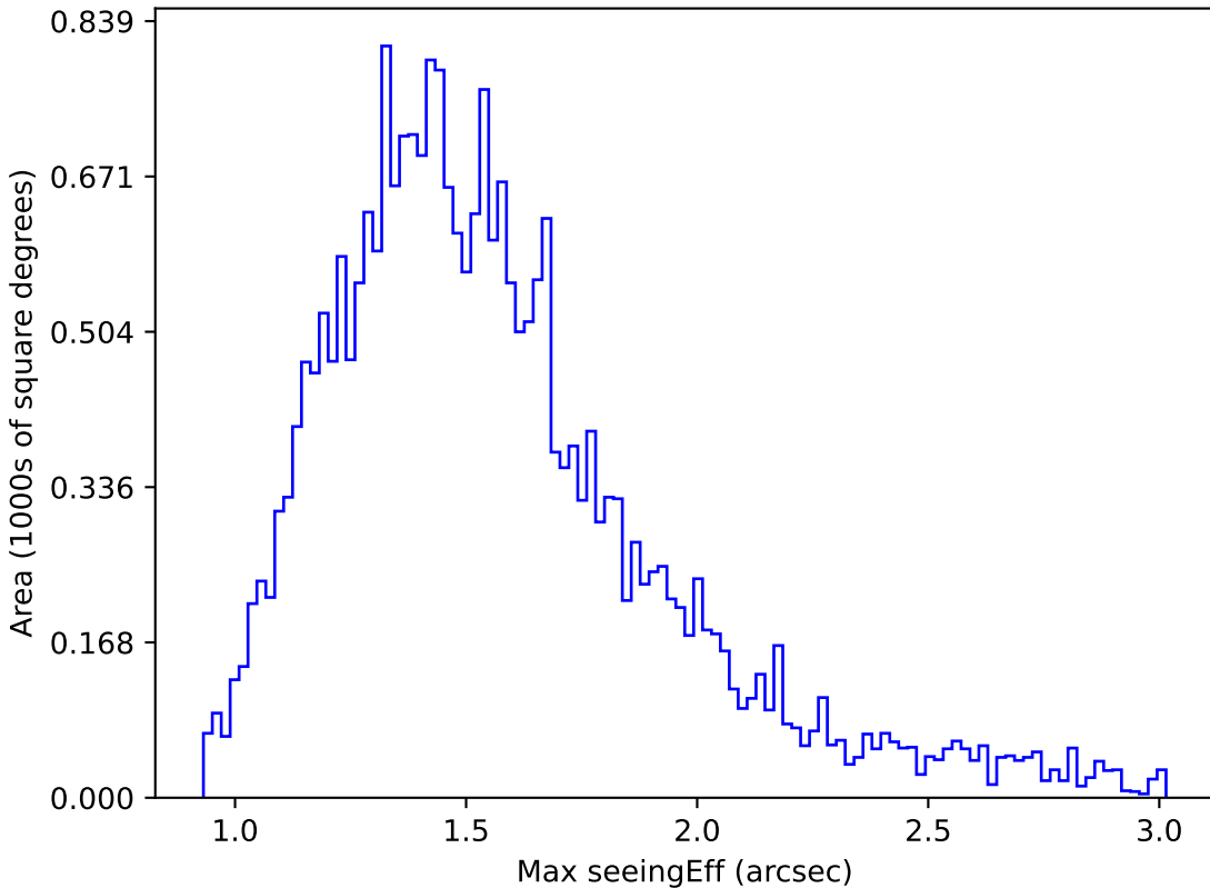
ddf_loaded_half_fl2_v3.4_10yrs Yr 1 z band: Max seeingEff
