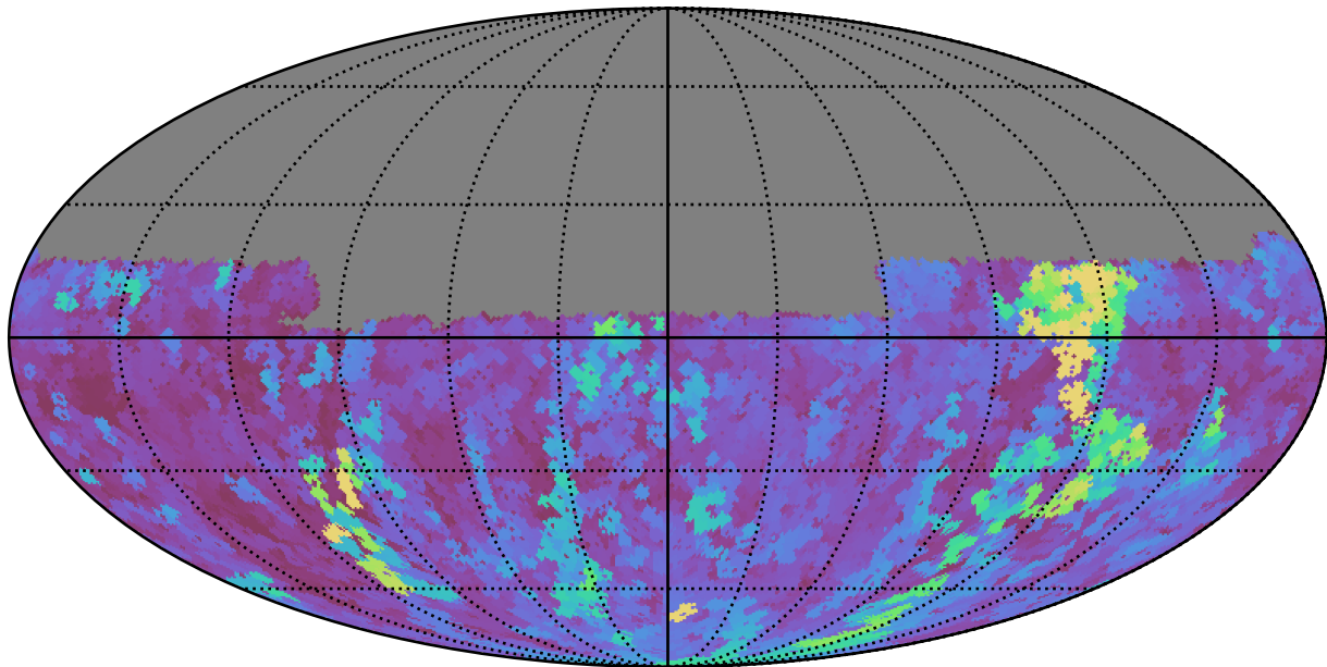
ddf_loaded_half_fl2_v3.4_10yrs Yr 1 u band: Max seeingEff
