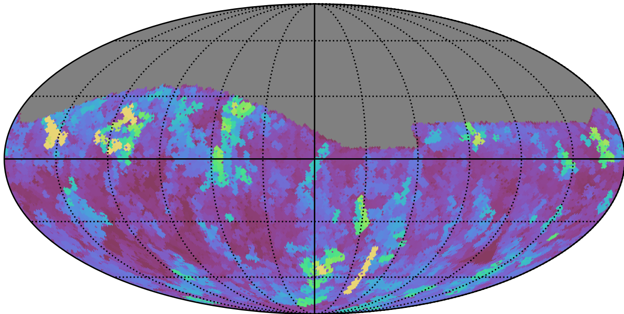
ddf_loaded_half_fl2_v3.4_10yrs Yr 1 i band: Max seeingEff
