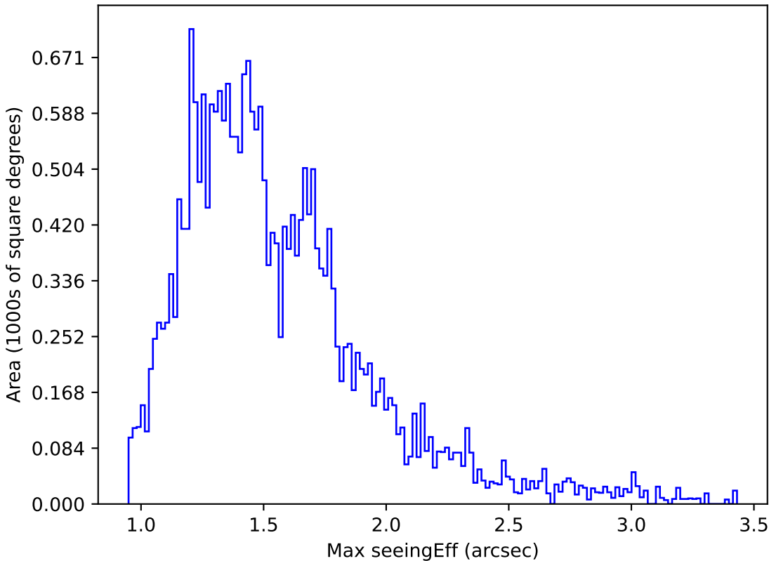
ddf_loaded_half_fl2_v3.4_10yrs Yr 1 i band: Max seeingEff
