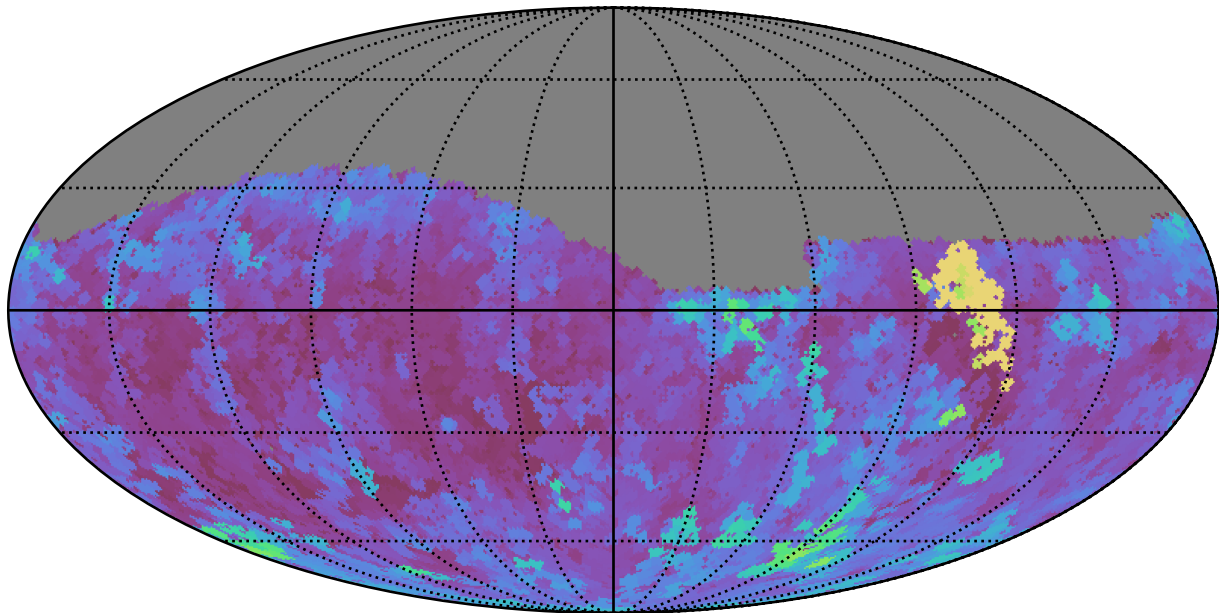
ddf_loaded_half_fl2_v3.4_10yrs Yr 1 g band: Max seeingEff
