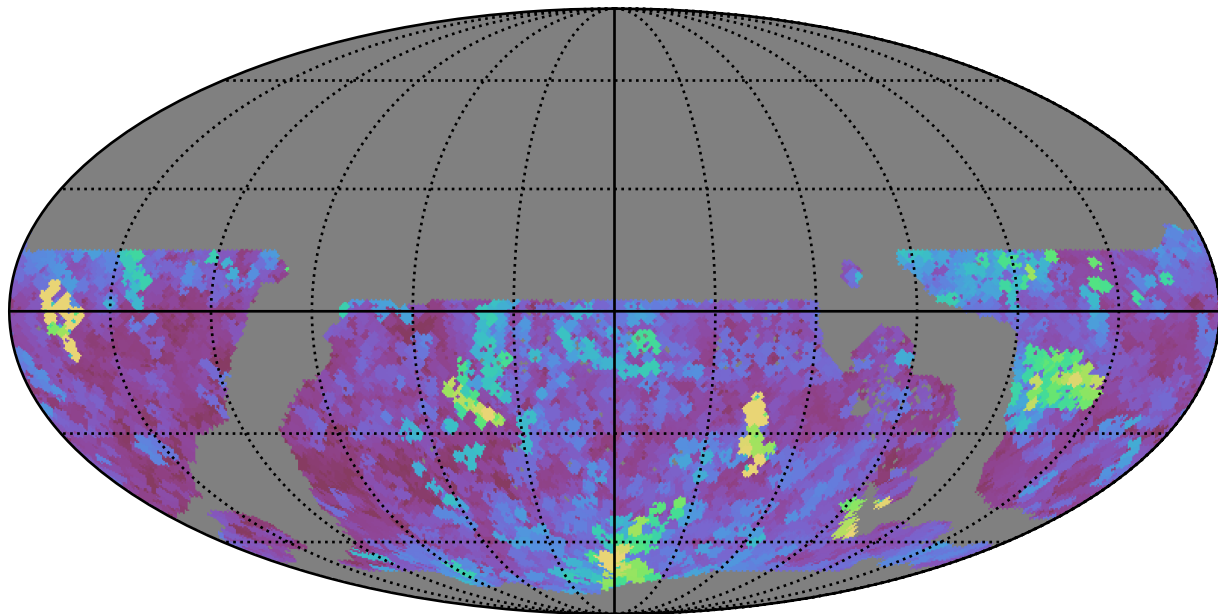
ddf_loaded_half_fl2_v3.4_10yrs WFD z band: Max seeingEff
