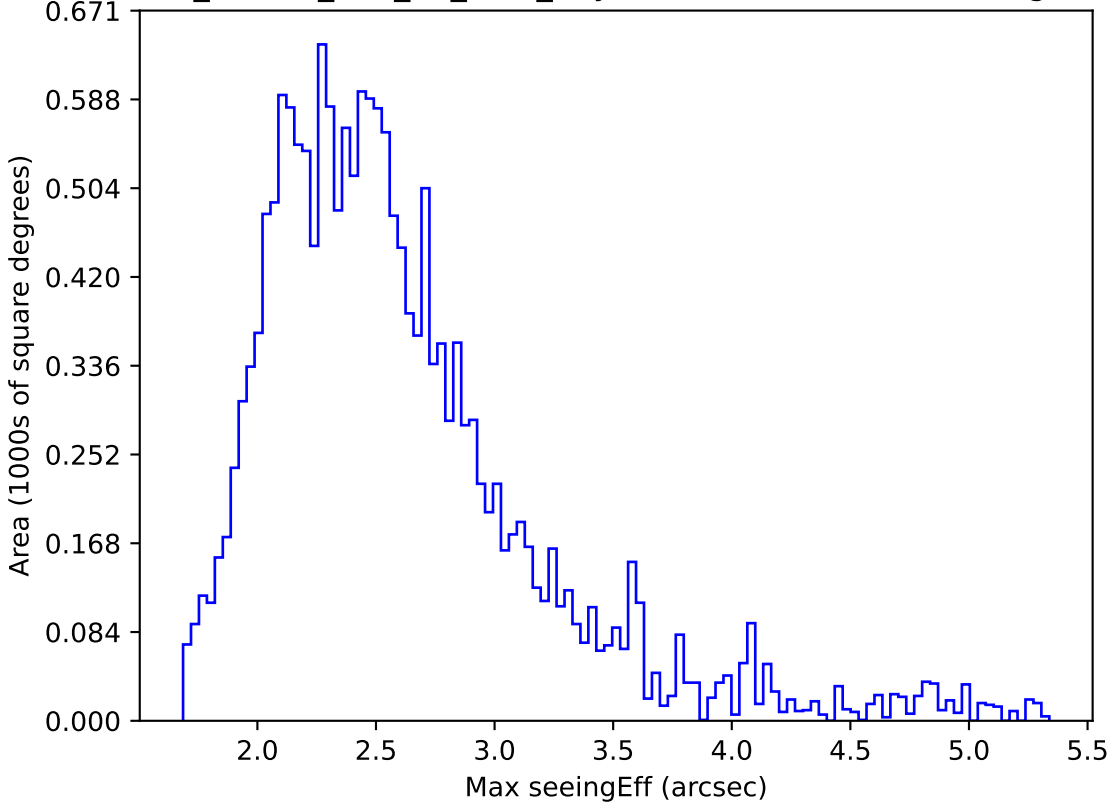
ddf_loaded_half_fl2_v3.4_10yrs WFD z band: Max seeingEff
