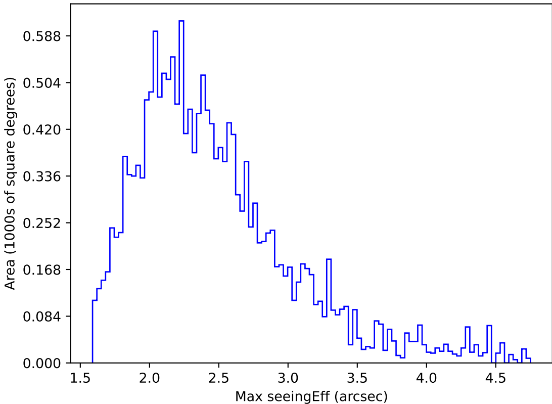
ddf_loaded_half_fl2_v3.4_10yrs WFD y band: Max seeingEff
