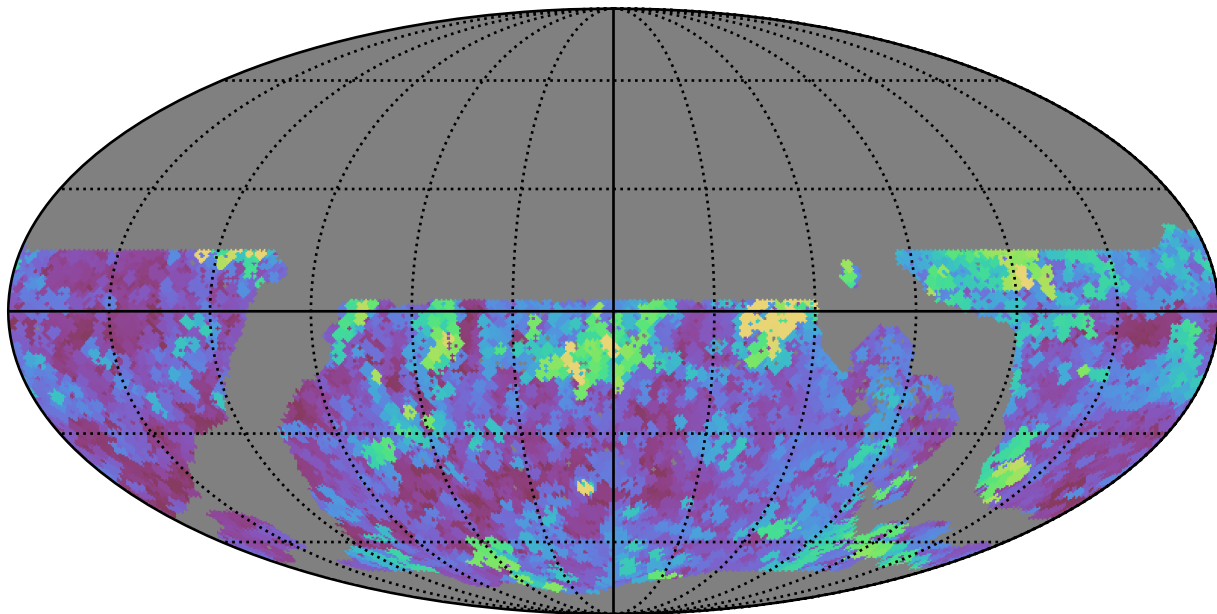
ddf_loaded_half_fl2_v3.4_10yrs WFD r band: Max seeingEff
