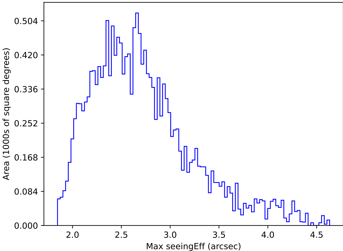
ddf_loaded_half_fl2_v3.4_10yrs WFD r band: Max seeingEff
