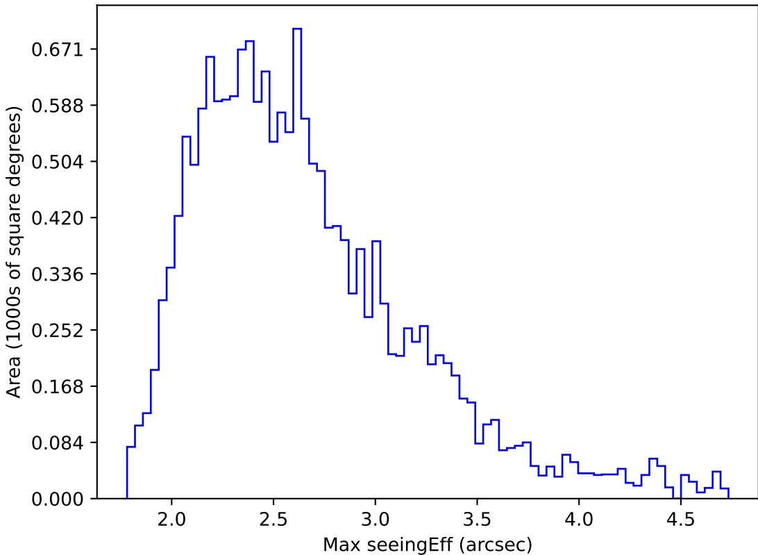
ddf_loaded_half_fl2_v3.4_10yrs WFD i band: Max seeingEff
