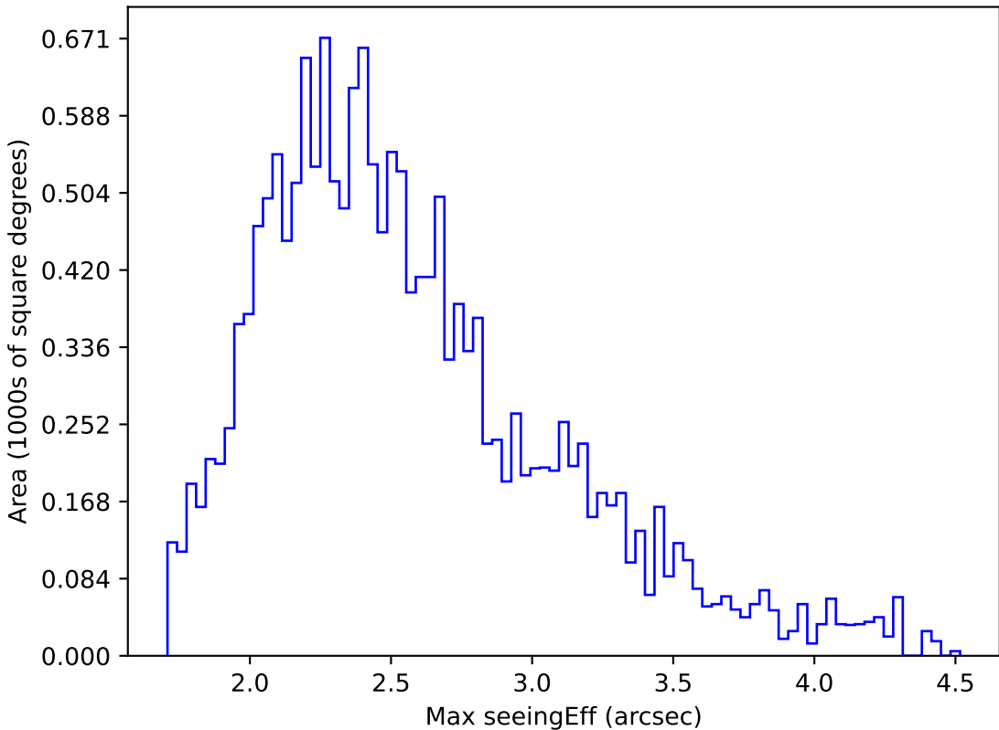
ddf_loaded_half_fl2_v3.4_10yrs WFD g band: Max seeingEff
