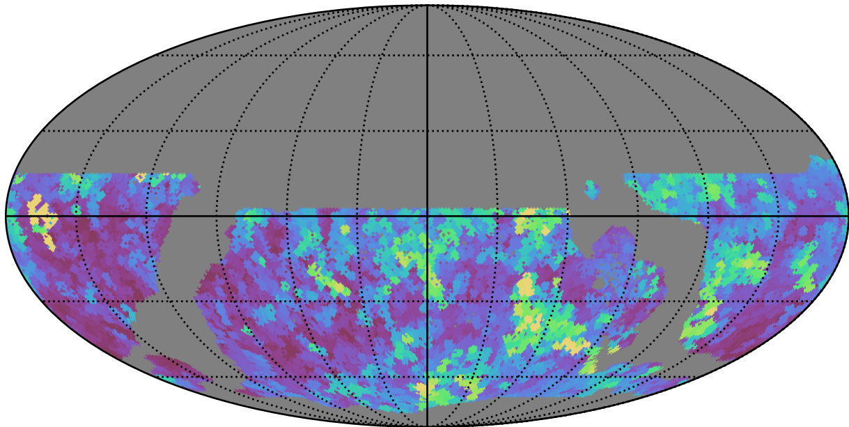
ddf_loaded_half_fl2_v3.4_10yrs WFD all bands: Max seeingEff
