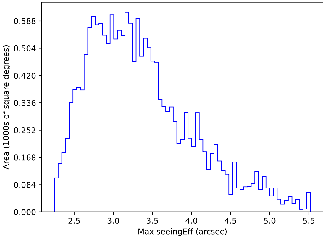
ddf_loaded_half_fl2_v3.4_10yrs WFD all bands: Max seeingEff
