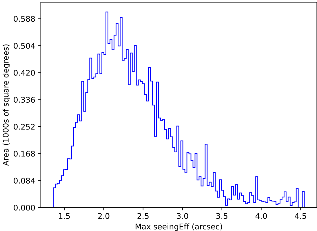
ddf_loaded_half_fl2_v3.4_10yrs All sky y band: Max seeingEff
