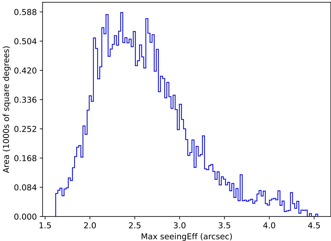
ddf_loaded_half_fl2_v3.4_10yrs All sky r band: Max seeingEff
