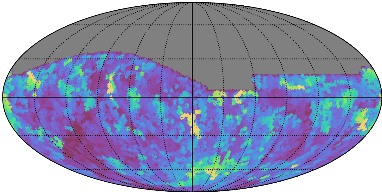
ddf_loaded_half_fl2_v3.4_10yrs All sky i band: Max seeingEff
