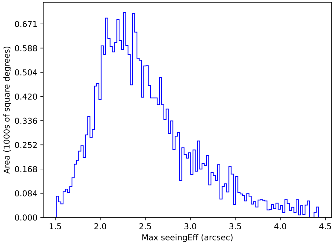
ddf_loaded_half_fl2_v3.4_10yrs All sky g band: Max seeingEff
