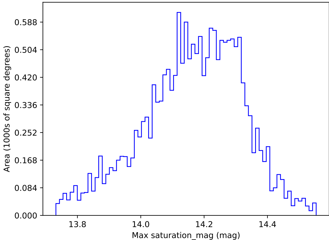
ddf_loaded_half_fl2_v3.4_10yrs WFD y band: Max saturation_mag
