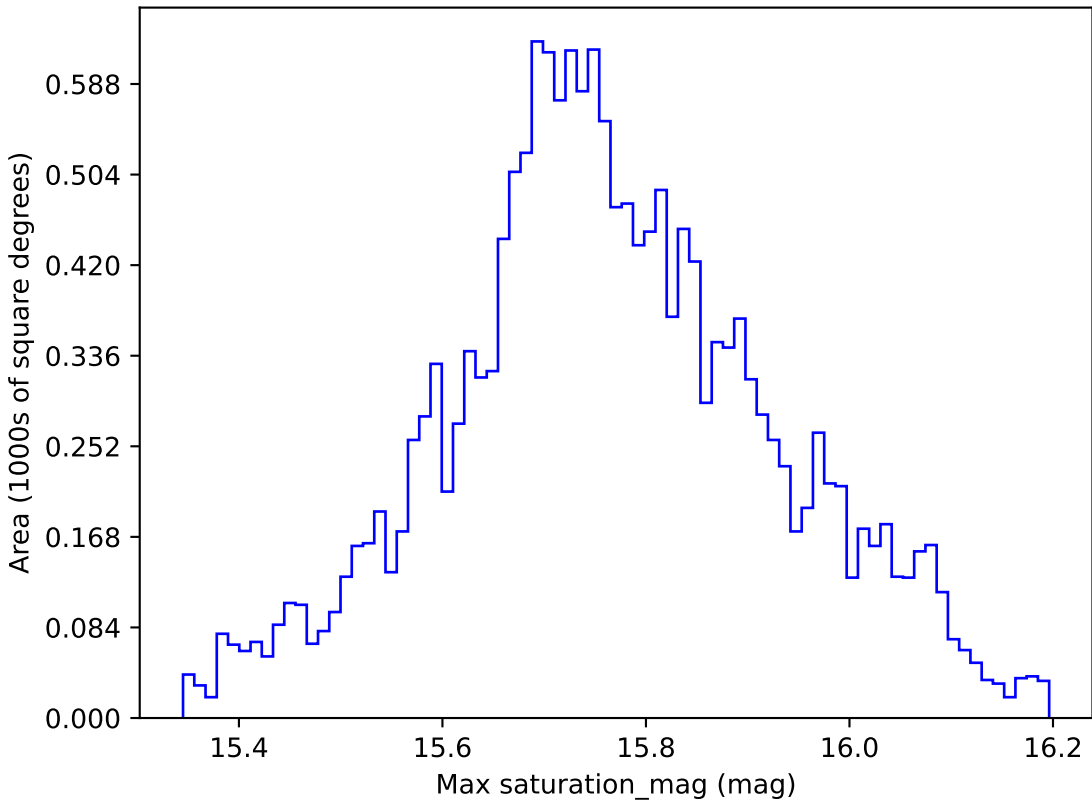
ddf_loaded_half_fl2_v3.4_10yrs WFD r band: Max saturation_mag
