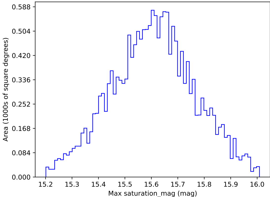
ddf_loaded_half_fl2_v3.4_10yrs WFD i band: Max saturation_mag
