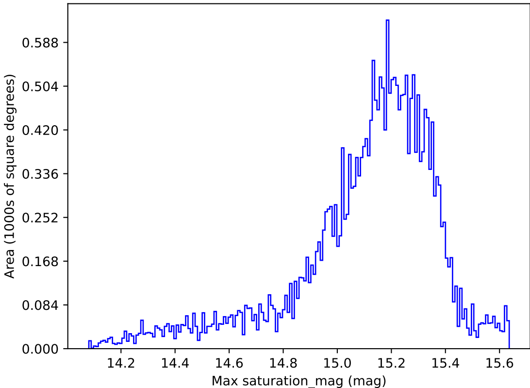
ddf_loaded_half_fl2_v3.4_10yrs All sky z band: Max saturation_mag
