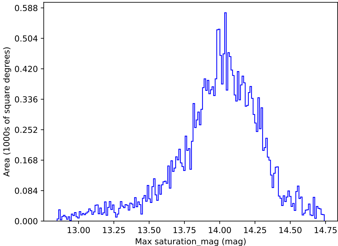
ddf_loaded_half_fl2_v3.4_10yrs All sky u band: Max saturation_mag
