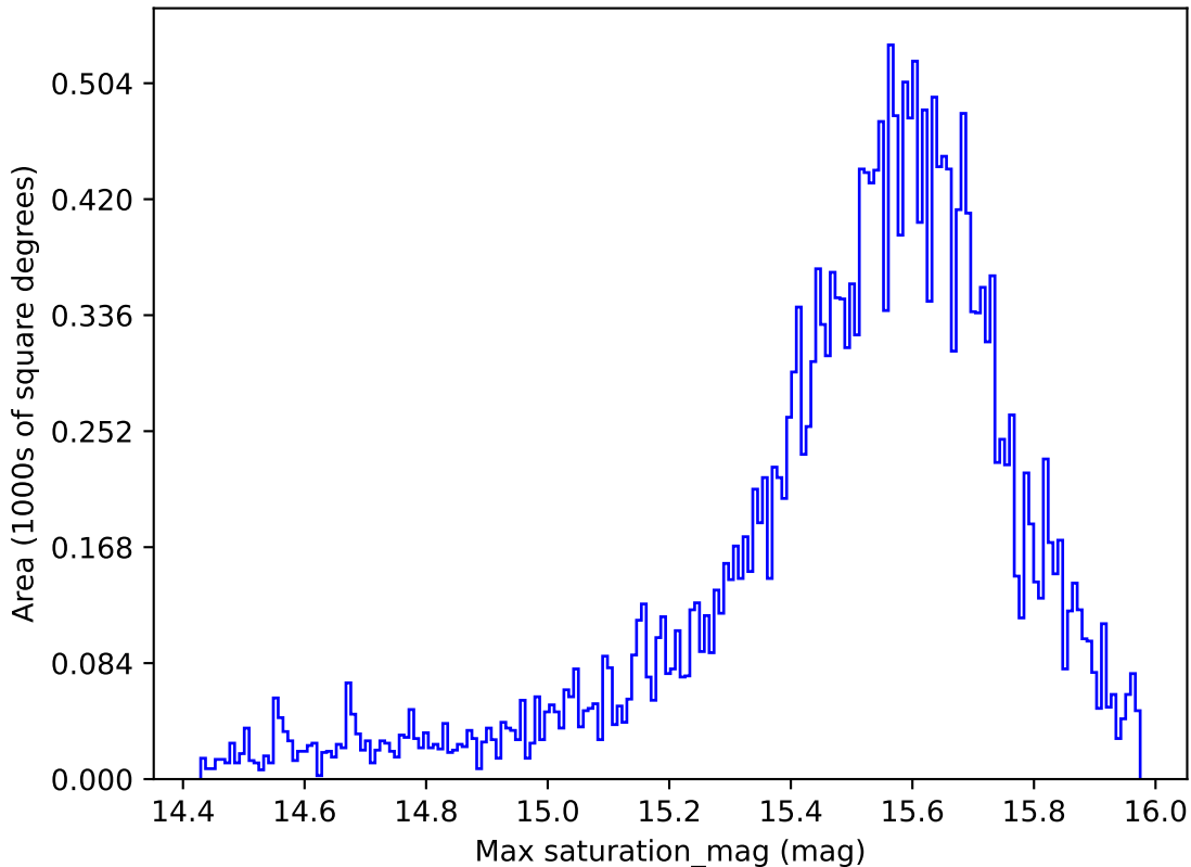
ddf_loaded_half_fl2_v3.4_10yrs All sky i band: Max saturation_mag
