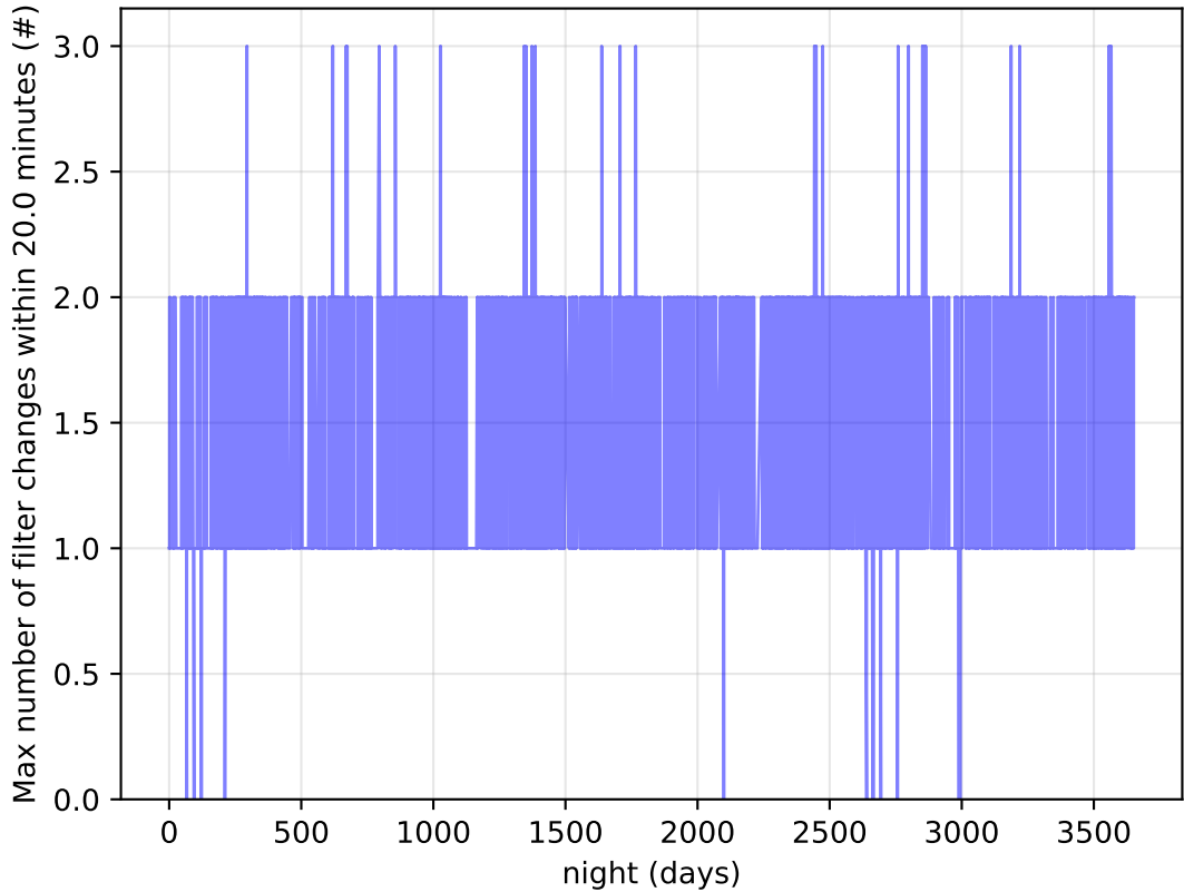
ddf_loaded_half_fl2_v3.4_10yrs Per Night: Max number of filter changes within 20.0 minutes
