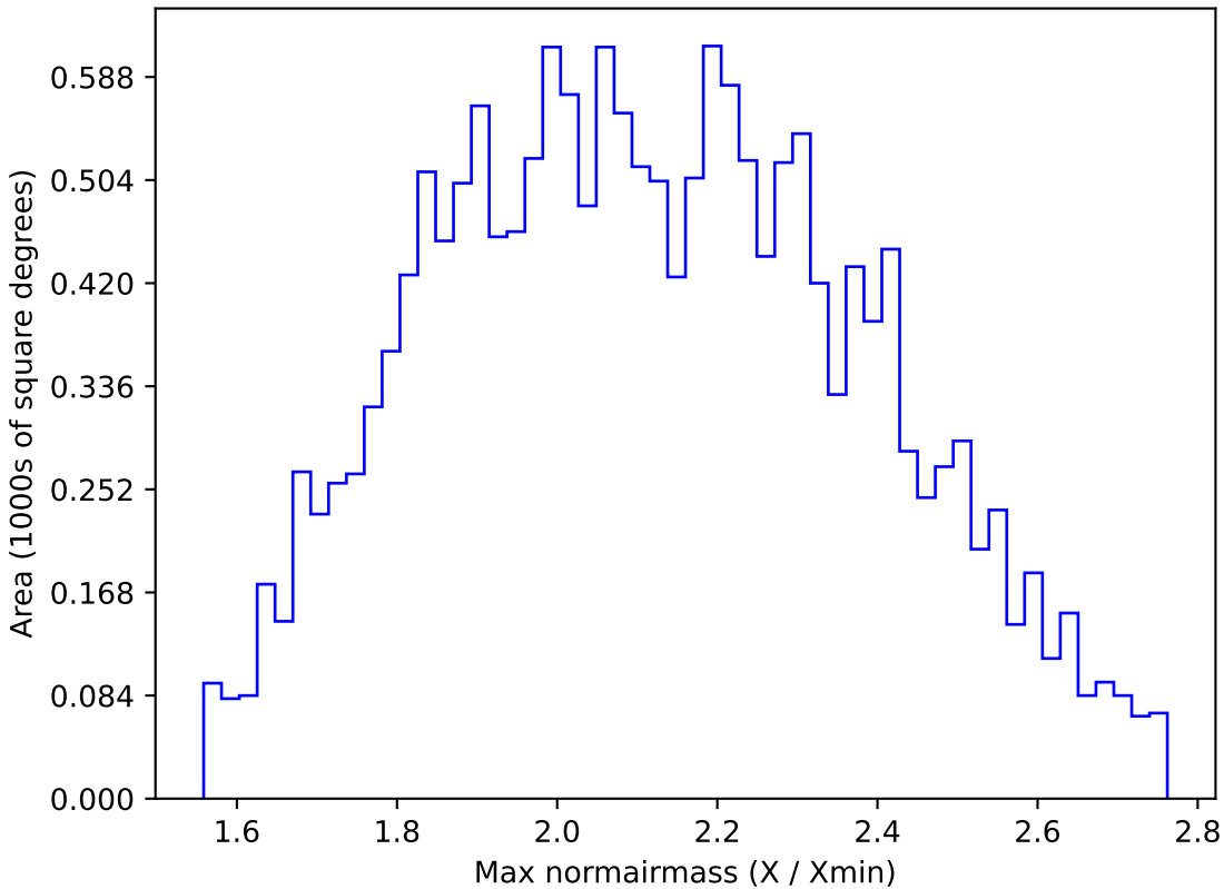
ddf_loaded_half_fl2_v3.4_10yrs WFD y band: Max normairmass
