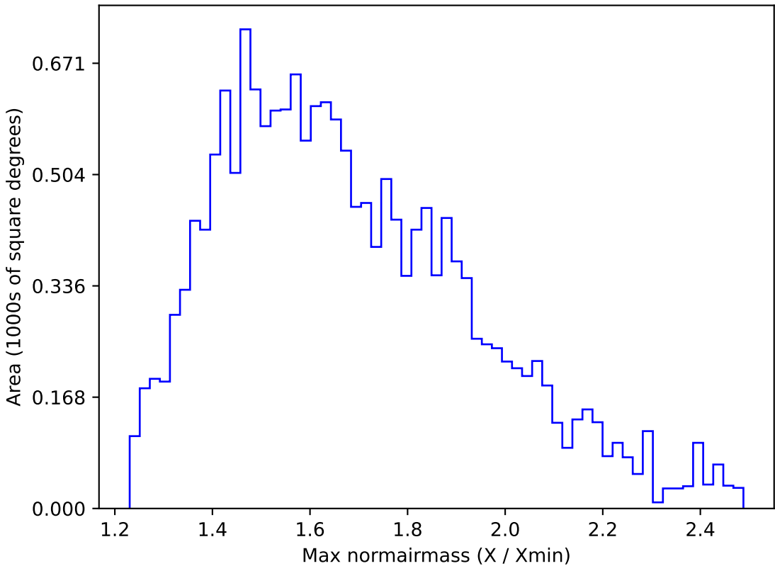
ddf_loaded_half_fl2_v3.4_10yrs WFD u band: Max normairmass
