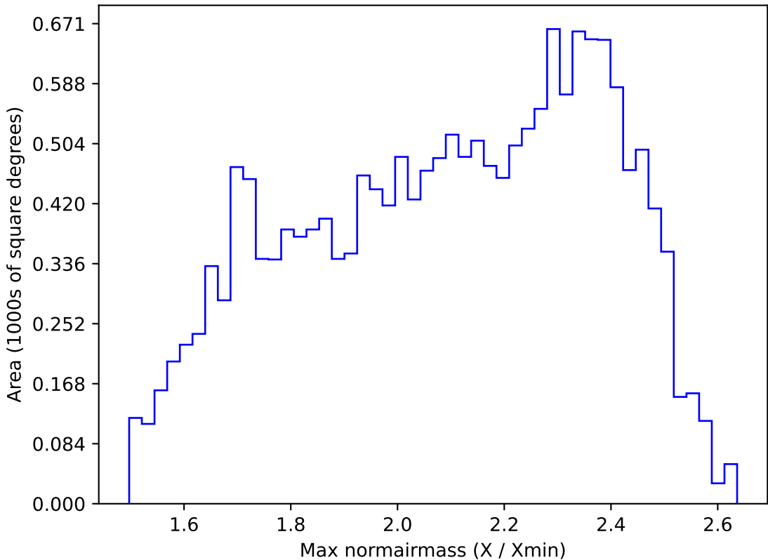
ddf_loaded_half_fl2_v3.4_10yrs WFD r band: Max normairmass
