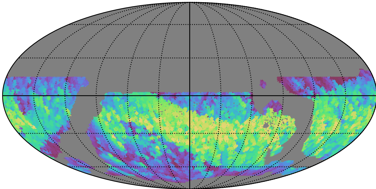
ddf_loaded_half_fl2_v3.4_10yrs WFD i band: Max normairmass
