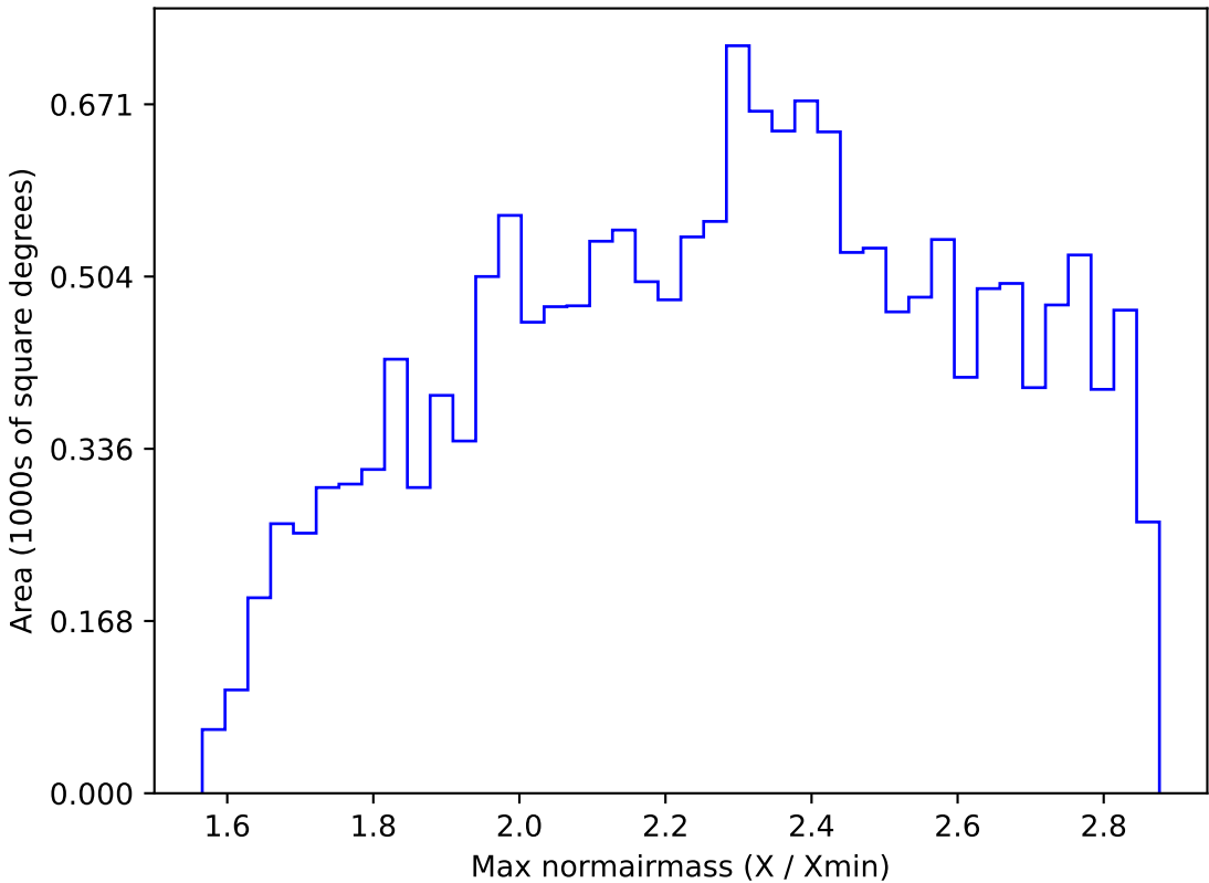
ddf_loaded_half_fl2_v3.4_10yrs WFD i band: Max normairmass
