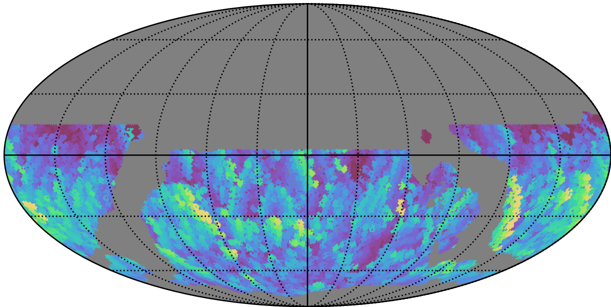
ddf_loaded_half_fl2_v3.4_10yrs WFD g band: Max normairmass
