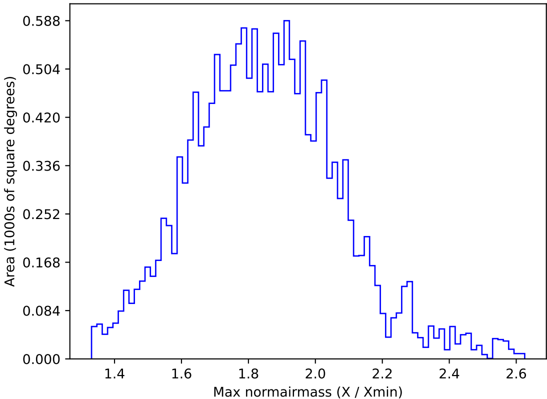
ddf_loaded_half_fl2_v3.4_10yrs WFD g band: Max normairmass
