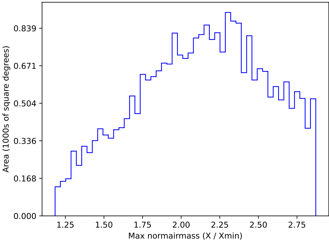
ddf_loaded_half_fl2_v3.4_10yrs All sky z band: Max normairmass
