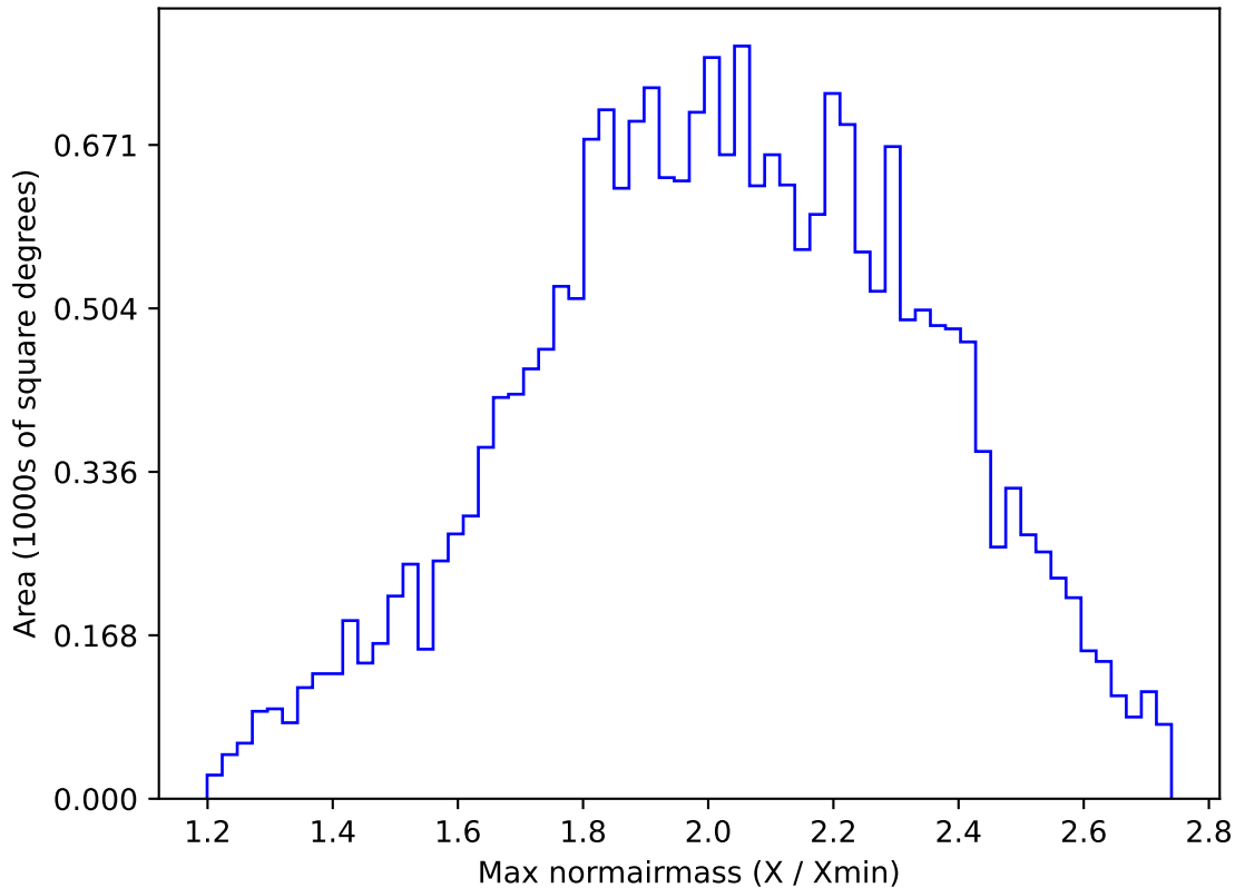
ddf_loaded_half_fl2_v3.4_10yrs All sky y band: Max normairmass
